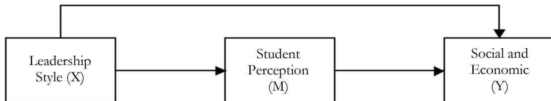
Chart 1. Hypothesis Model
