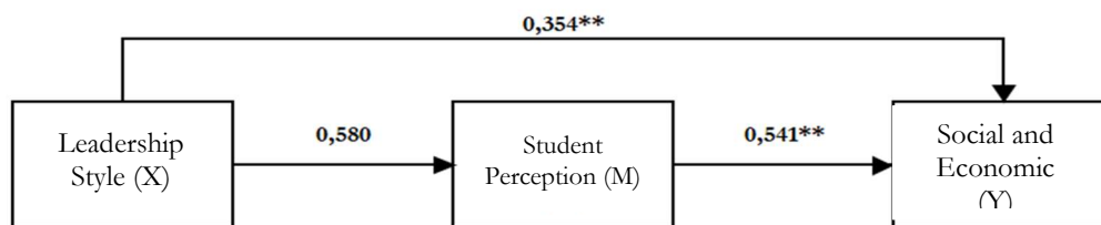
Chart 2. Test-Path Analysis
